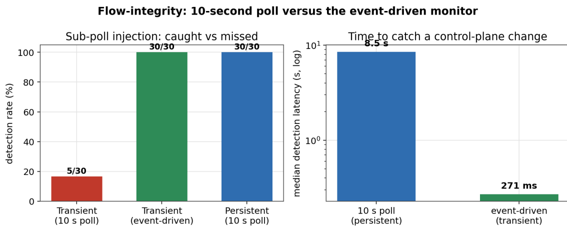
Figure A.14: Flow-integrity, ten-second poll versus the event-driven monitor. Left: a two-second transient injection is missed by the poll on 25 of 30 trials but caught on all 30 by the event-driven monitor; a persistent injection is caught by both. Right: median detection latency, 8.5s for the poll against 0.27s for the monitor (log axis). Sources: results/flowint/{persistent,transient}.csv , results/gap4-flowmonitor/transient_eventdriven.csv .
