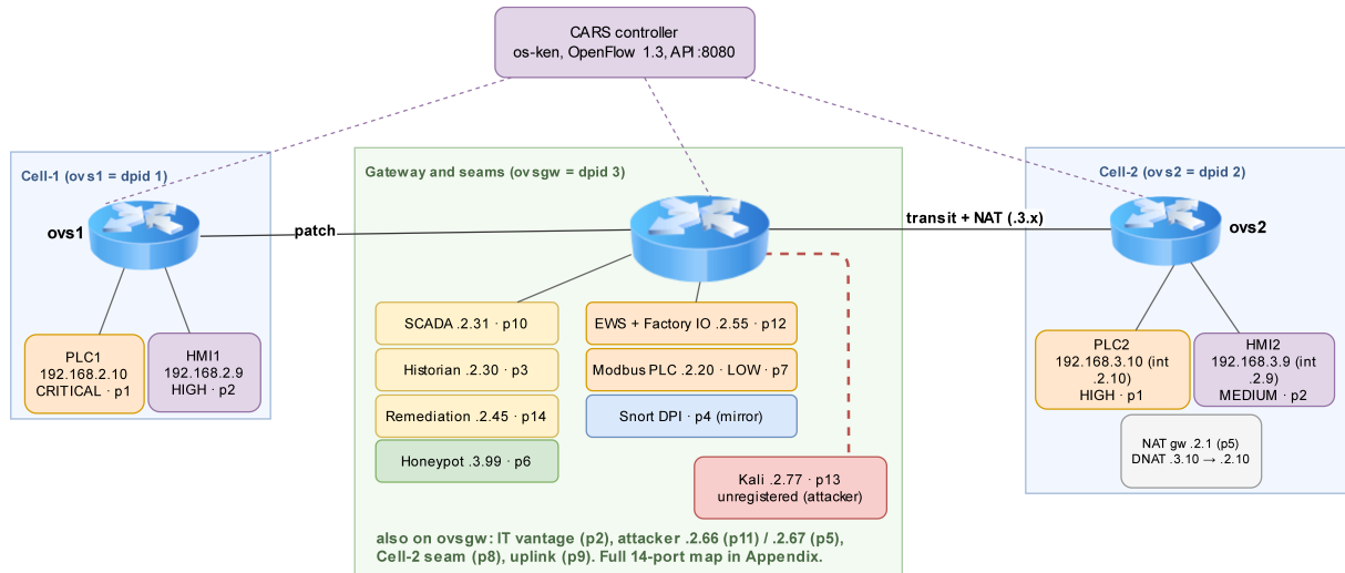
Figure 3.1: The SDN-ICS testbed topology. Three OpenFlow switches under a single controller: Cell-1 on ovs1 , the gateway on ovsgw , and Cell-2 on ovs2 , the last reached through a NAT clone. Addresses, criticality tiers and ofports are read from the running fabric; the full port and binding map is in Appendix A.
