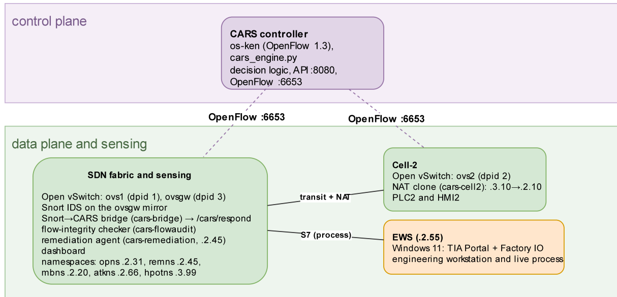
Figure 3.13: Deployment. The controller governs the three switches ( ovs1 , ovsgw , ovs2 ) over the OpenFlow control plane; the fabric, the Snort sensor and the supporting agents run together, and the engineering workstation with Factory IO is the live process.
