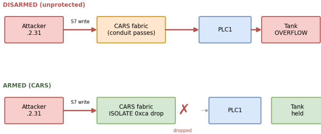
Figure 4.2: The path of a malicious S7 write in each state. Disarmed, the write crosses the fabric, reaches PLC1 and drives the tank to overflow. Armed, the reactive rule ( cookie 0x00ca ) drops it in the fabric, so it never reaches the PLC and the process is held.
