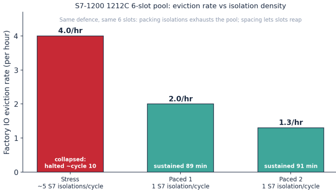
Figure A.21: The S7-1200 (1212C) connection-pool limit. The CPU exposes six dynamic connection resources; repeatedly isolating S7 sessions leaves half-open sessions that consume them. Packing about five isolations into each short cycle evicted the legitimate Factory IO client at 4.0 times an hour and the run could not be sustained; pacing to one isolation per cycle held the process for about ninety minutes at 1.3 to 2.0 evictions an hour. This is the empirical confirmation of the connection-pool caveat in Section 4.12. Source: night_*/logs/{freeze,monitor,mttm_all}.csv .
