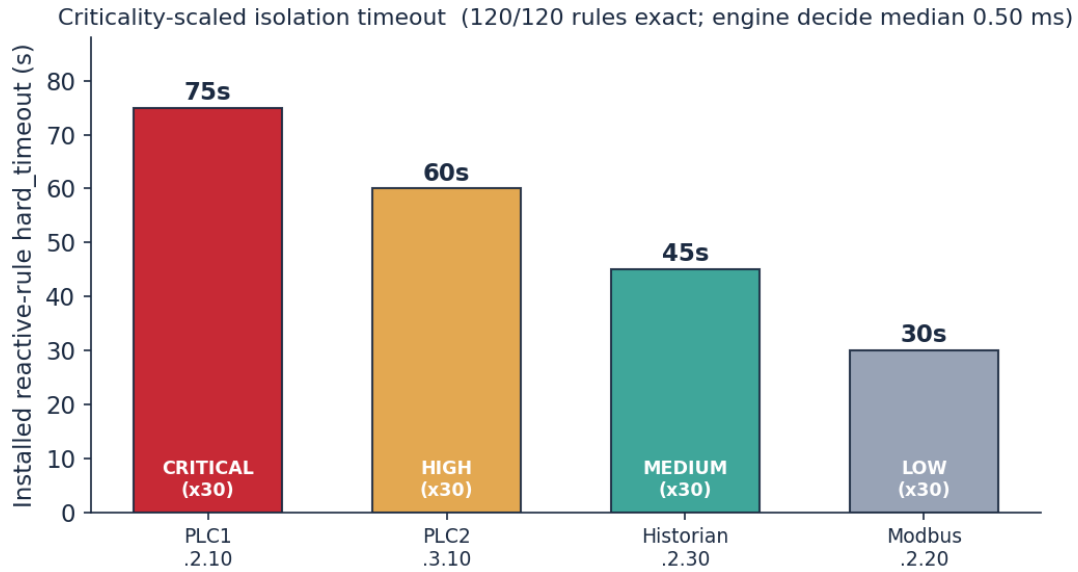
Figure A.20: Criticality-scaled isolation timeout over 120 tier probes across the four runs. Every probe installed 75/60/45/30s for CRITICAL/HIGH/MEDIUM/LOW with no deviation, at a median engine decide-time of 0.50 ms. Source: night_*/logs/tierladder.csv .
