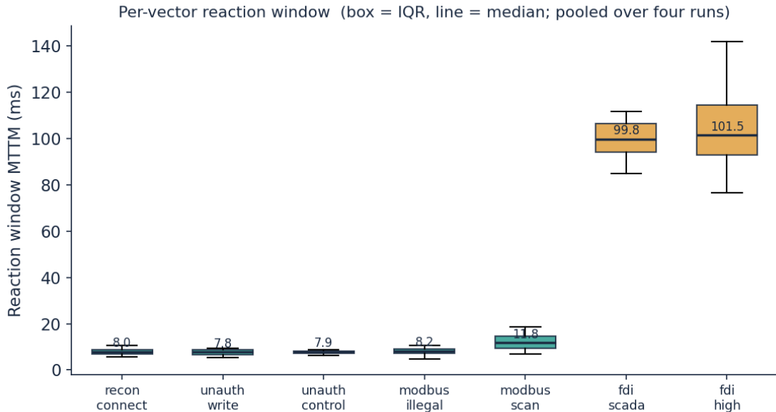
Figure A.19: Per-vector reaction window pooled over the four runs (box is the interquartile range, line the median). The source-cut vectors sit at roughly 7 to 12 ms; the two false-data injection vectors from the compromised trusted host sit near 100 ms because they draw a conduit block rather than an immediate source cut. Source: night_*/logs/mttm_all.csv .
