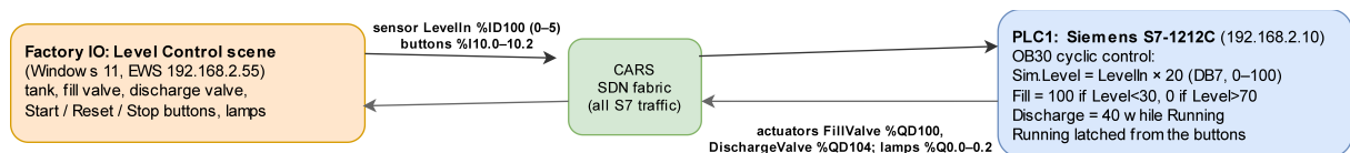
Figure 3.4: The hardware-in-the-loop. Factory IO supplies the level and button inputs and renders the valve and lamp outputs; PLC1 runs the control in OB30; every exchange crosses the CARS fabric. Addresses and mappings are from the deployed project.
