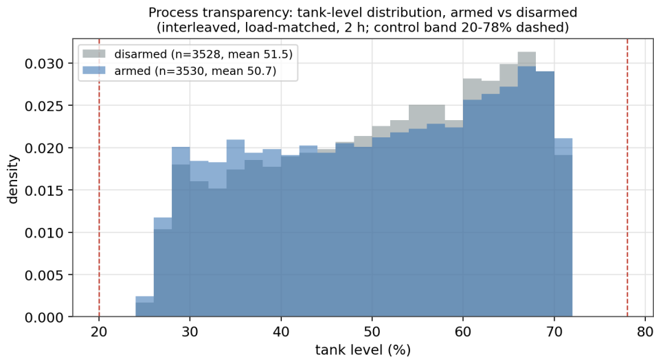
Figure A.15: Process transparency: the tank-level distribution armed against disarmed, over roughly seven thousand interleaved, load-matched per-second samples. The two distributions coincide (means 51.5 against 50.7%) and neither leaves the control band, so arming the defence has no measurable effect on the process. Source: results/e2/interleaved.csv .
