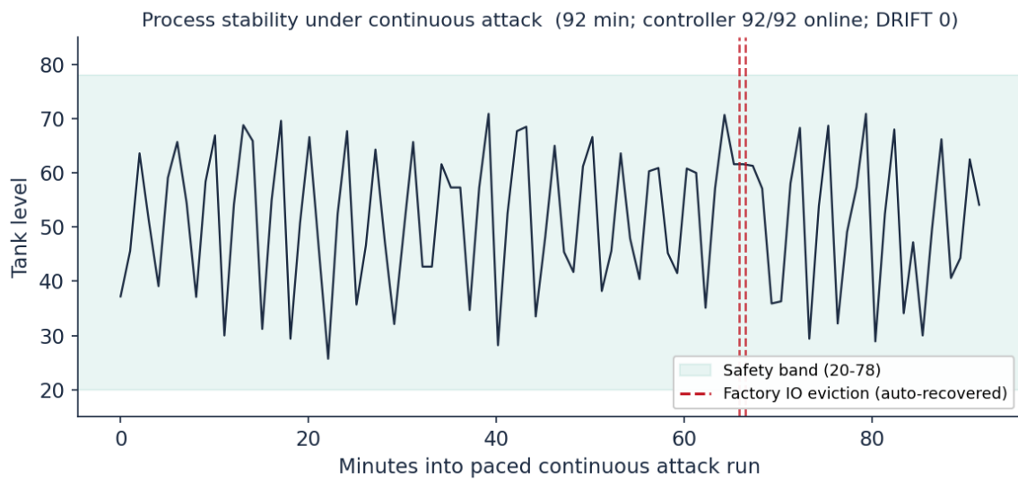
Figure A.22: Process stability under continuous attack: the tank level across the ninety-two-minute paced run, held within the 20 to 78 control band throughout. The controller and its remediation agent reported the process online in all ninety-two one-minute snapshots (this is the agent's PLC link sampled once a minute, which does not capture sub-minute client outages) and the flow auditor reported no drift. The two dashed marks are the brief Factory IO client evictions that the liveness guard caught and recovered. Source: night_paw2.0153/logs/{monitor,freeze}.csv .
