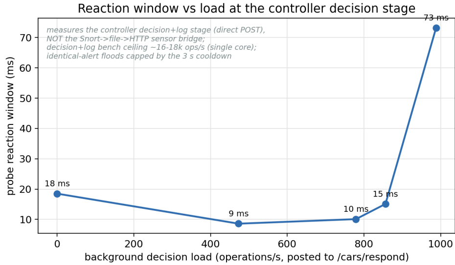
Figure A.16: Reaction window against background load, measured at the controller’s decision-and-log stage: both the background and the probe are posted directly to /cars/respond , so this characterises the controller ( classify , select_response and the audit write), not the Snort-to-file-to-HTTP sensor bridge. The window holds in the tens of milliseconds to about a thousand operations a second and rises only as this single-threaded stage nears its sixteen-to-eighteen-thousand-a-second bench ceiling. The sensor bridge is a separate and lower ceiling, the acknowledged bottleneck carried to the future work (Section 4.12), and is not what this curve measures. Source: results/gap1_live/curve.csv .
