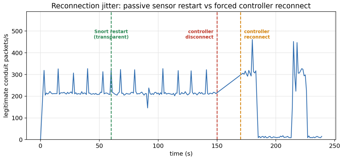
Figure A.17: Reconnection jitter on the legitimate conduit: restarting the passive Snort sensor is transparent (no dip), whereas a forced controller reconnection stalls forwarding. Source: results/jitter/timeline.csv (one spurious counter sample removed).
