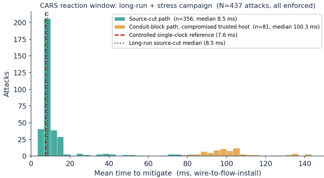
Figure A.18: Reaction window over the long-run and stress campaign. The source-cut path (356 attacks, median 8.5 ms) sits close to the 7.6 ms controlled single-clock reference of Section 4.6; the false-data injections from the compromised trusted host form a separate mode near 100 ms, the conduit-block path that installs after the first packets. 437 of the 440 measured attacks are shown: two under-load DDoS-probe samples, which belong to the load curve rather than the clean reaction window, and one physically impossible negative row from a stale-rule read, are excluded. Source: the four night_*/logs/mttm_all.csv .
