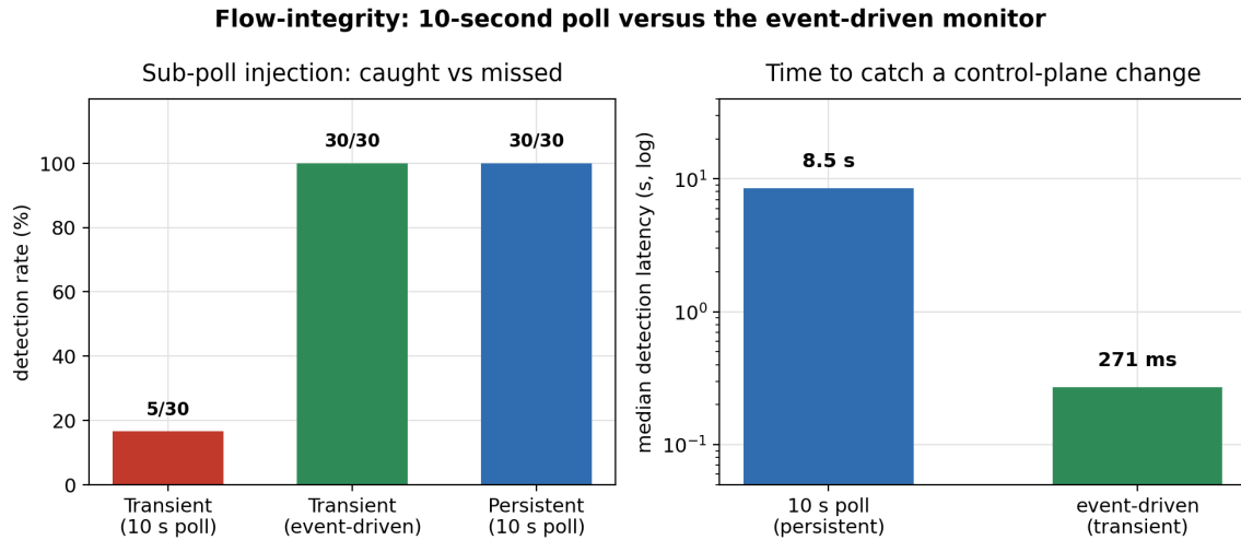
Figure A.14: Flow-integrity, ten-second poll versus the event-driven monitor. Left: a two-second transient injection is missed by the poll on 25 of 30 trials but caught on all 30 by the event-driven monitor; a persistent injection is caught by both. Right: median detection latency, 8.5s for the poll against 0.27s for the monitor (log axis). Sources: results/flowint/{persistent,transient}.csv , results/gap4-flowmonitor/transient_eventdriven.csv .
