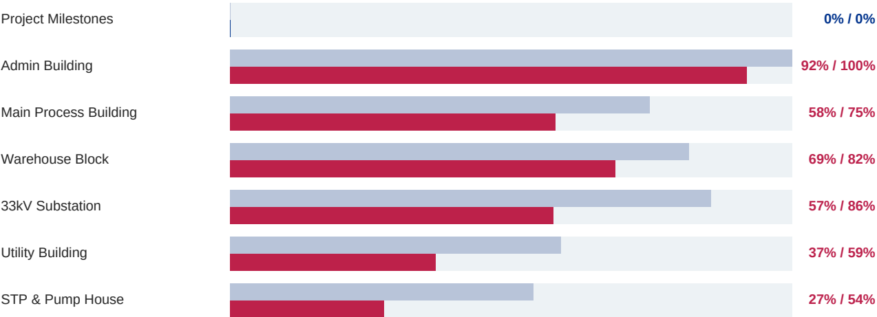
Building-wise progress (planned vs actual)
