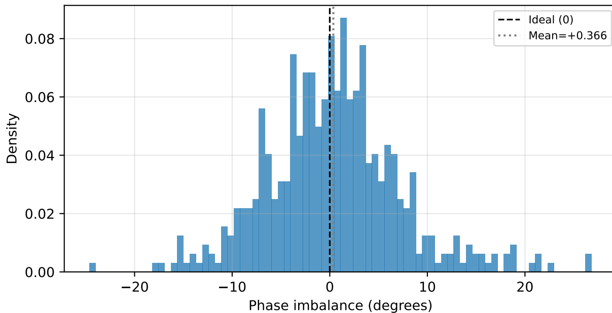
USRP B200 RX Phase imbalance (degrees)
