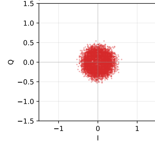
(b) Constellation — RTL-SDR V3 RX
