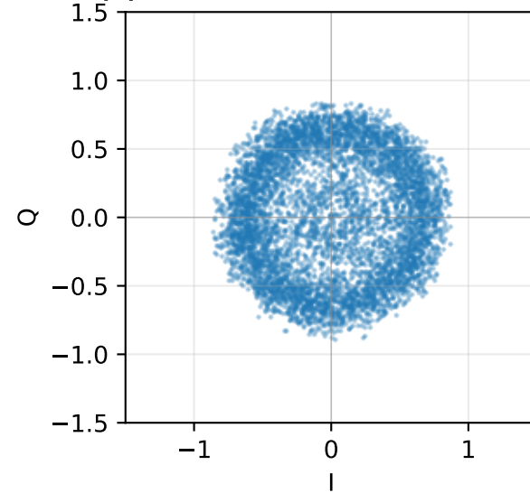
(b) Constellation — USRP B200 RX
