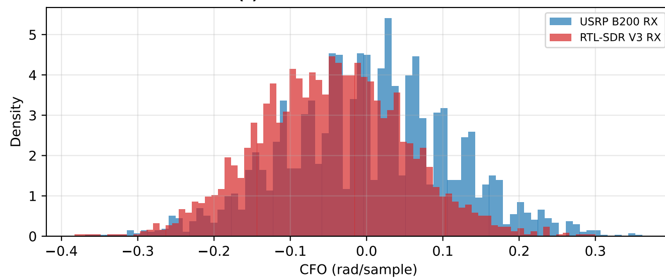
(c) CFO distribution KS=0.2177
