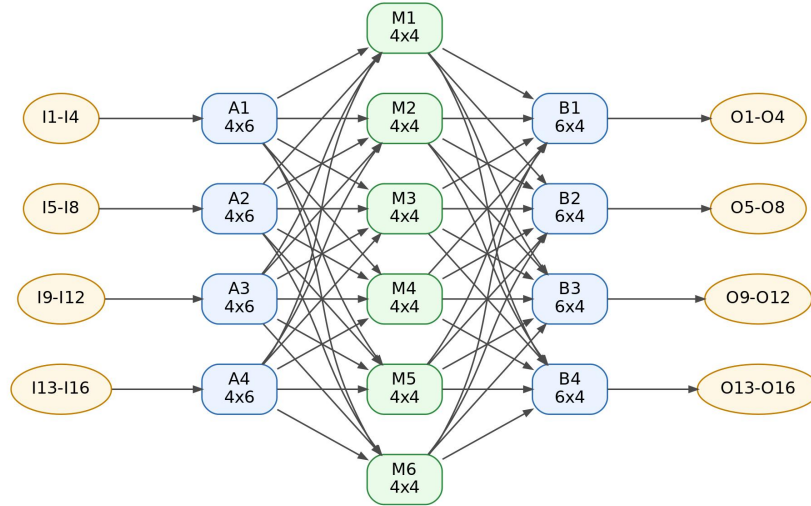
Figure 1: 3-stage Clos network diagram ( N=16 , n=4 , k=6 , m=4 )
