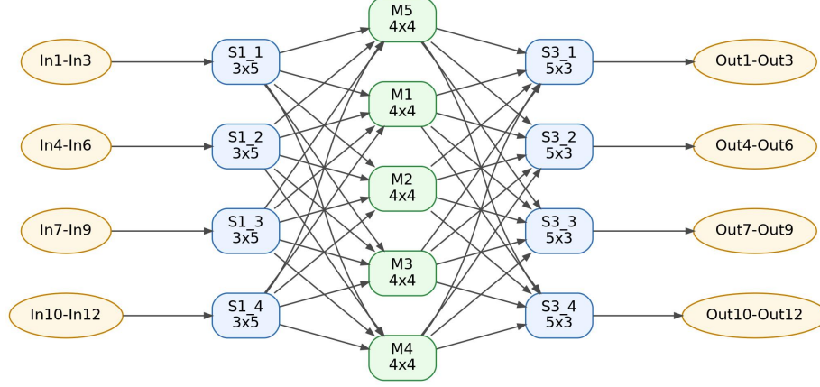
Figure 1: 3-stage Clos network diagram ( N=12 , n=3 , k=5 , m=4 )
