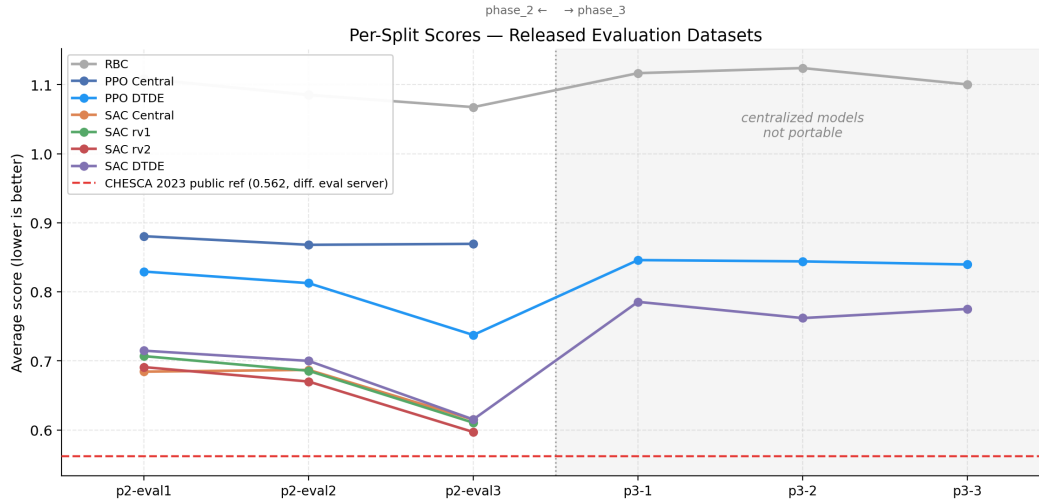
Figure 2: Released held-out scores across phase-2 (3 buildings) and phase-3 (6 buildings). Centralized policies cannot run on phase-3; SAC-DTDE is the best portable phase-3 policy. The dashed line is the CHESCA 2023 leaderboard reference.
