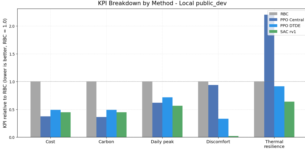
Figure 4: KPI breakdown on local public_dev, normalized relative to RBC (RBC = 1; lower is better). RL improves thermal discomfort most sharply; thermal-resilience loss remains the main residual weakness.
