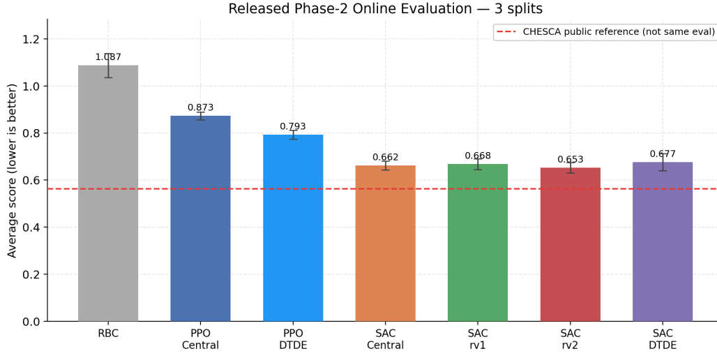
Figure 3: Released phase-2 comparison. Bars aggregate three held-out 3-building splits; error bars show 95% confidence intervals over evaluation jobs. SAC reward_v2 is the best single-checkpoint policy.
