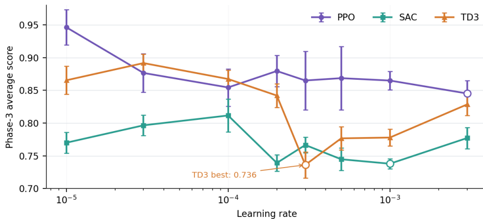
Figure 5: Broad learning-rate screen on released phase-3 transfer splits. Each point aggregates three seeds over three 6-building splits; TD3 peaks at 3 \times 10^{-4} .
