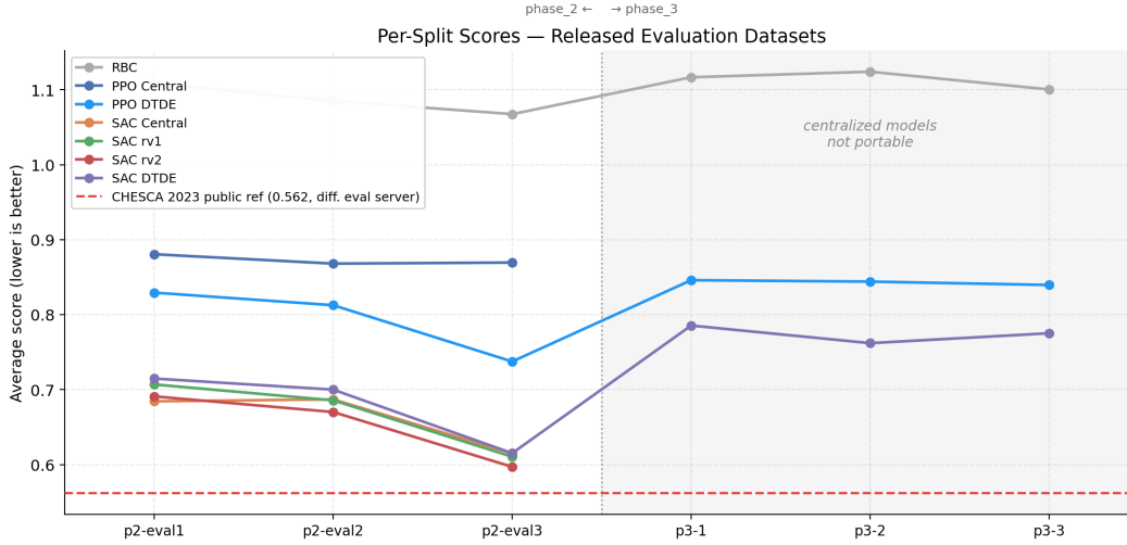
Figure 2: Released held-out scores across phase-2 (3 buildings) and phase-3 (6 buildings). Centralized policies cannot run on phase-3; SAC-DTDE is the best portable phase-3 policy. The dashed line is the CHESCA 2023 leaderboard reference.
