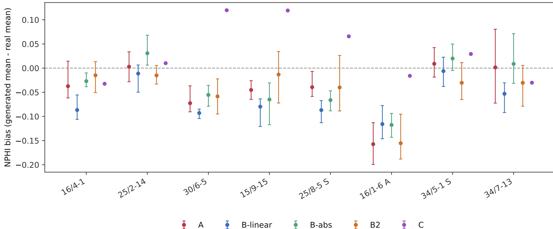
F1: per-well NPHI bias, 8 wells x 5 arms (error bars: min/max across 5 within-well realizations, descriptive only)
