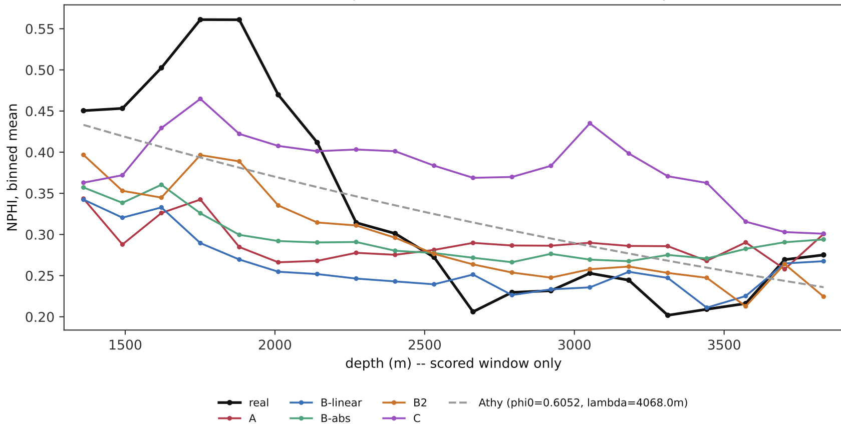
F3: NPHI vs depth, binned means, scored window only
