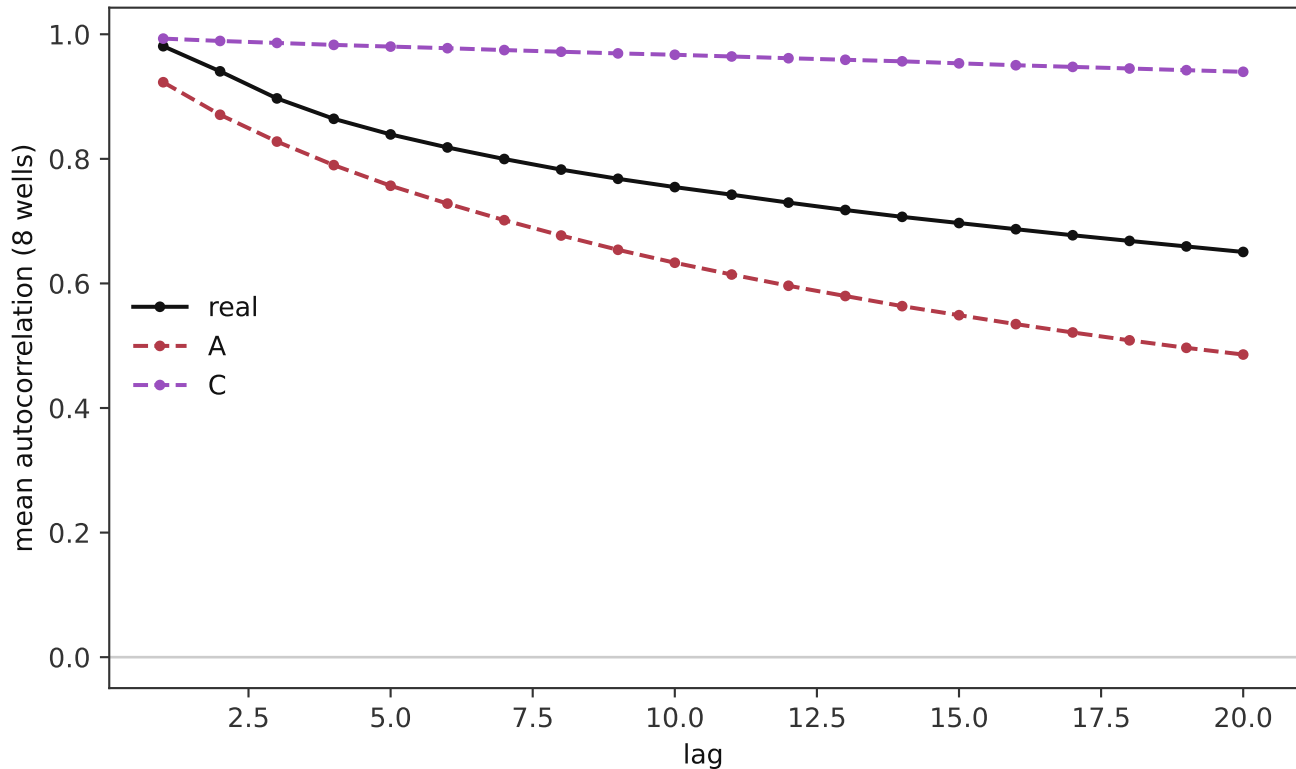
F4: NPHI autocorrelation, lags 1-20
