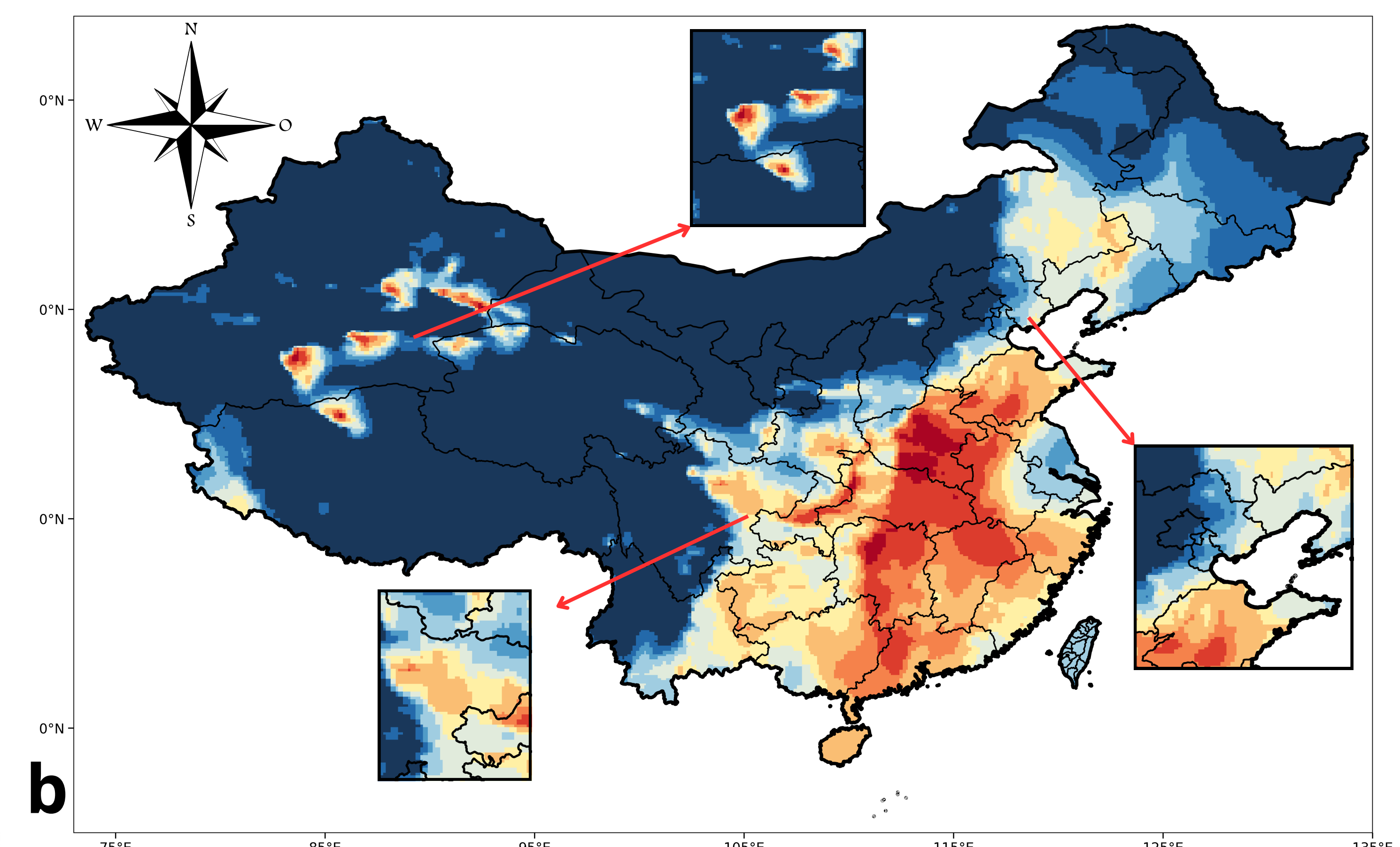
TopoFlow PM 2.5 predictions
