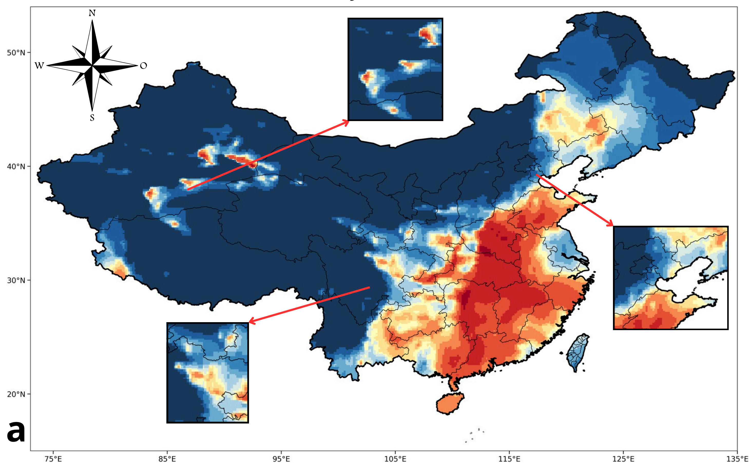
Ground truth (CAQRA reanalysis): Ground-based PM 2.5 observations
