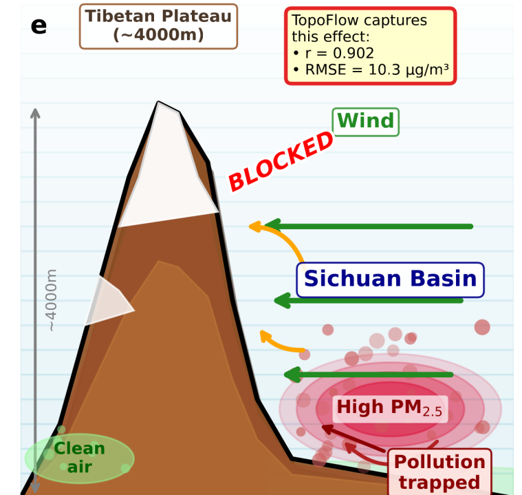
Conceptual: Topographic blocking mechanism
