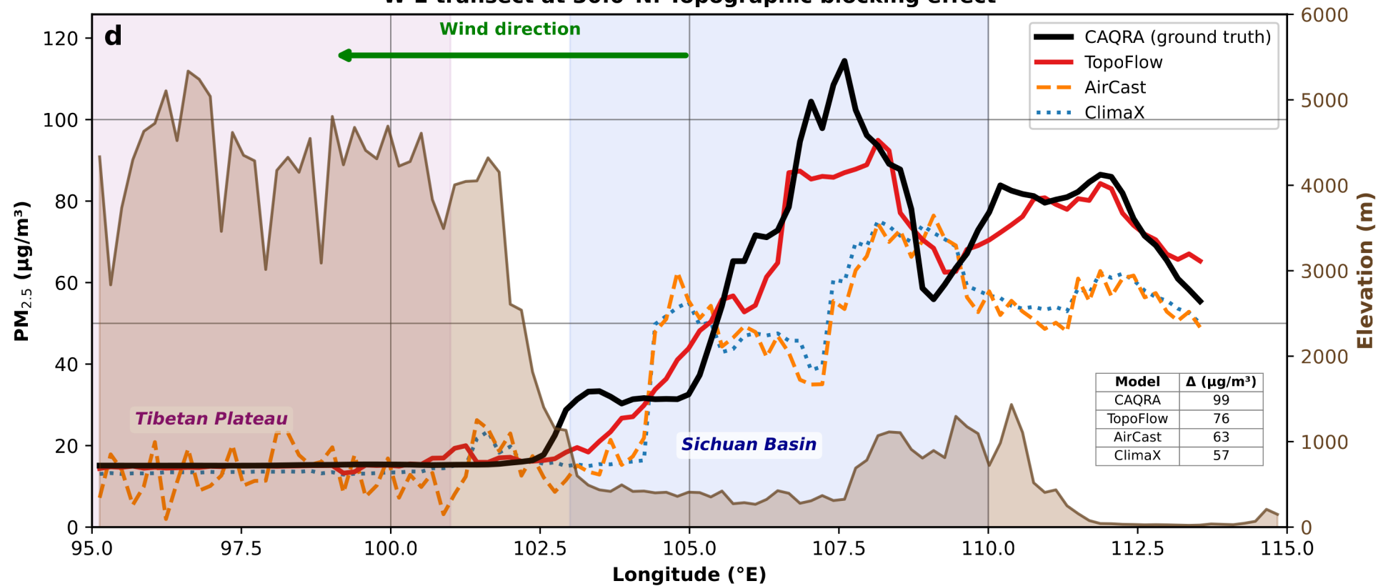
W-E transect at 30.0°N: Topographic blocking effect
