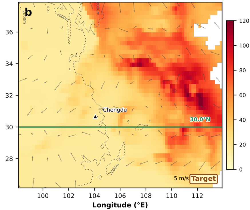
CAQRA (ground truth) (t = 0h), 8 July 2018 08:00 UTC
