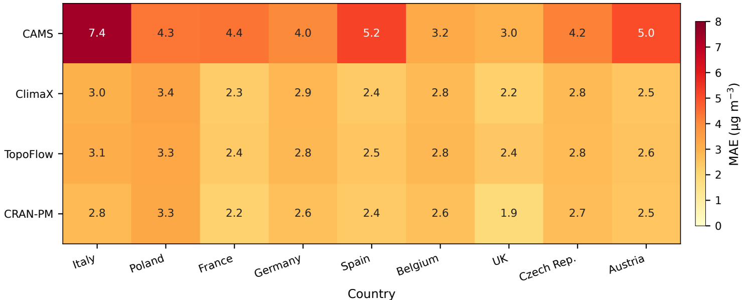
Per-country MAE ( \mu\text{g m}^{-3} ), T+1, EEA stations 2022
