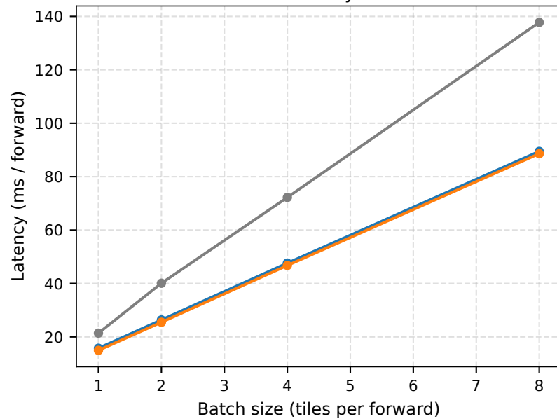
Latency
