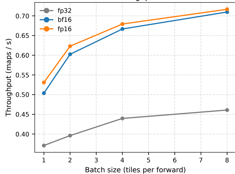
Throughput
