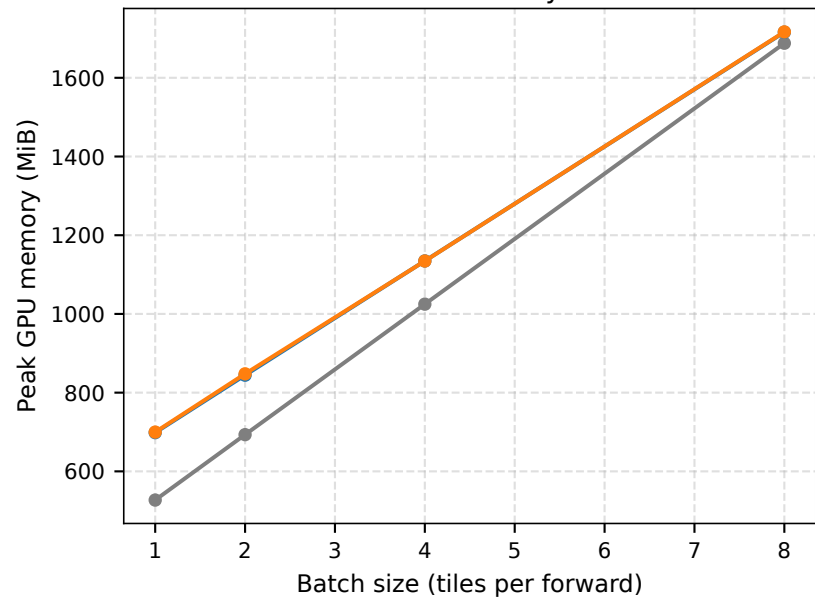
Peak memory
