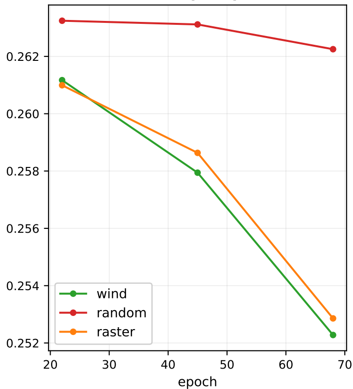
Val loss (per epoch)
