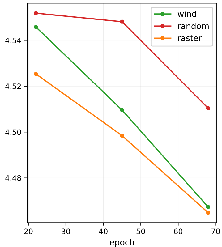
Val RMSE ( \mu\text{g m}^{-3} , per epoch)
