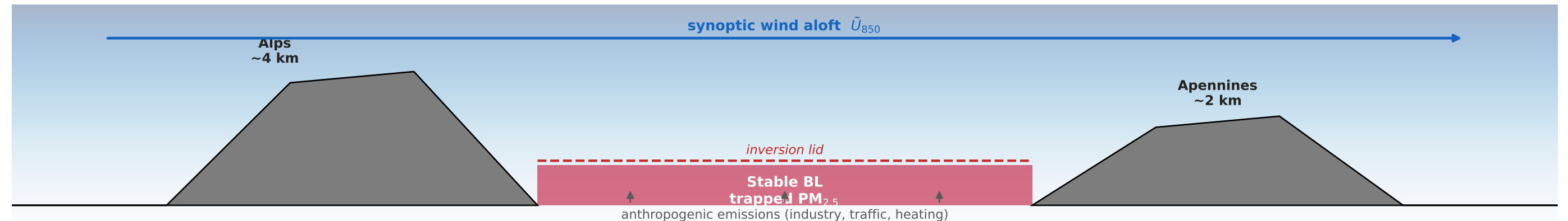
(e) Conceptual model : stable boundary layer over the Po Plain, bounded by Alps (N) and Apennines (S)
