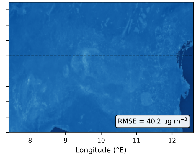
(c) CRAN-PM T+1 — Po Valley
