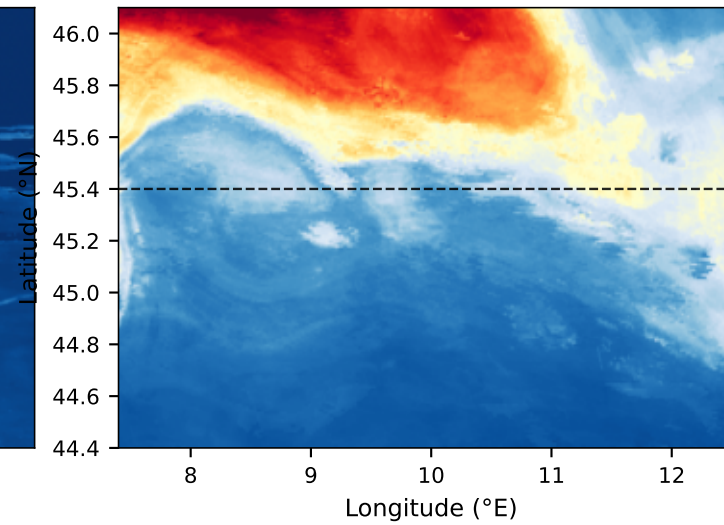
(b) GHAP truth — Po Valley
