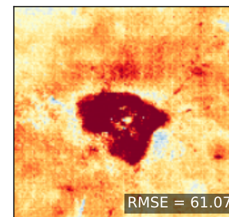
CRAN-PM T+1
