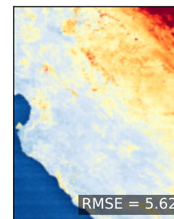
CRAN-PM T+1
