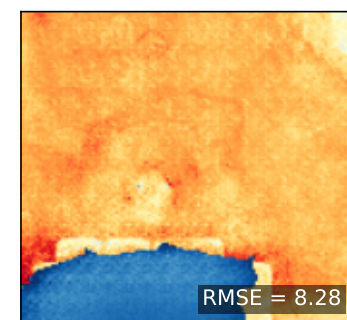
CRAN-PM T+1
