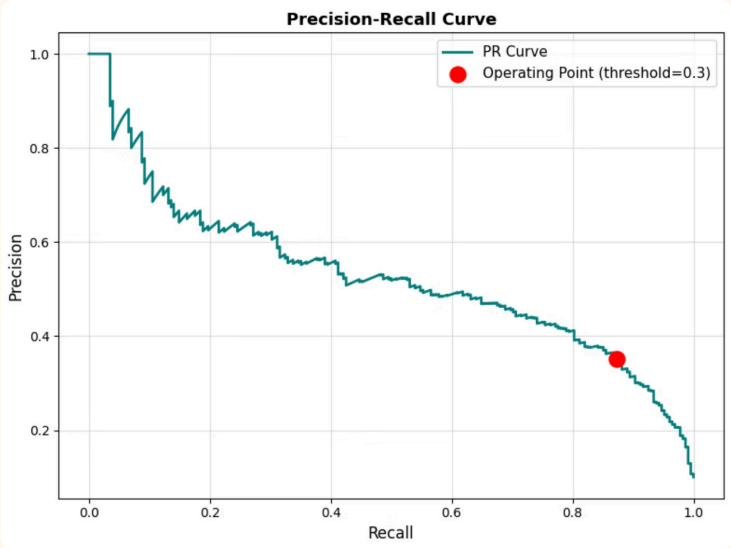
Precision Recall Curve (threshold @0.3)
