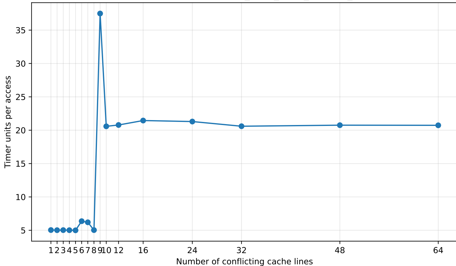
Hazel associativity sweep: AMD_EPYC_9654_96-Core_Processor
