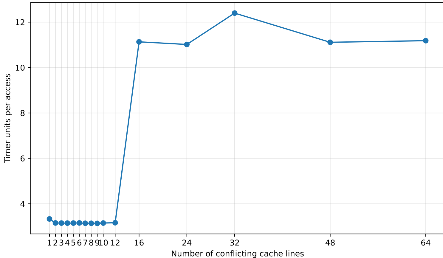
Hazel associativity sweep: AMD_EPYC_9655_96-Core_Processor
