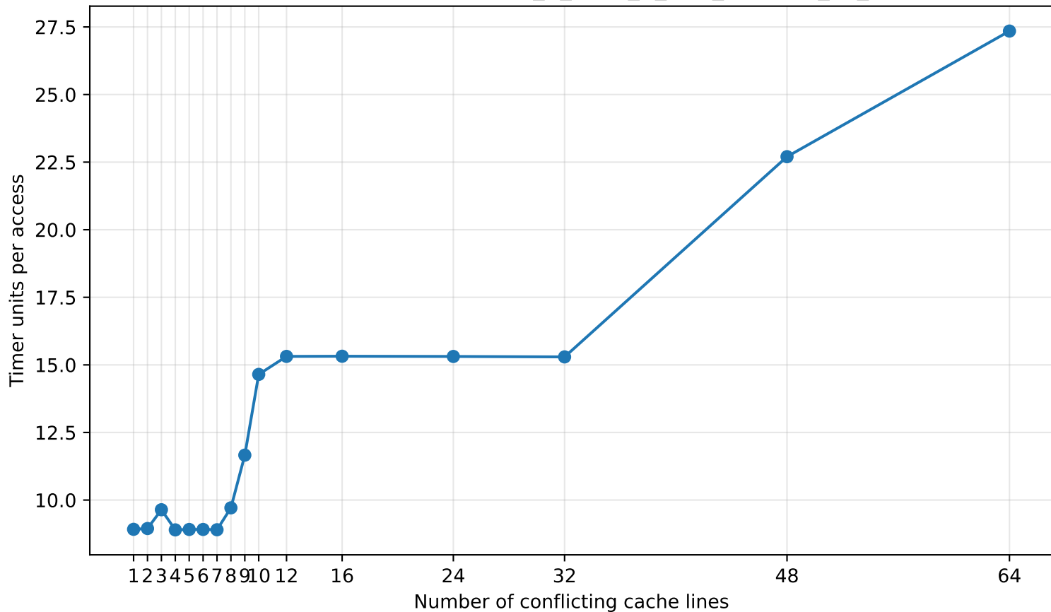
Hazel associativity sweep: Intel_R_Xeon_R_CPU_E5-2650_v3_2.30GHz
