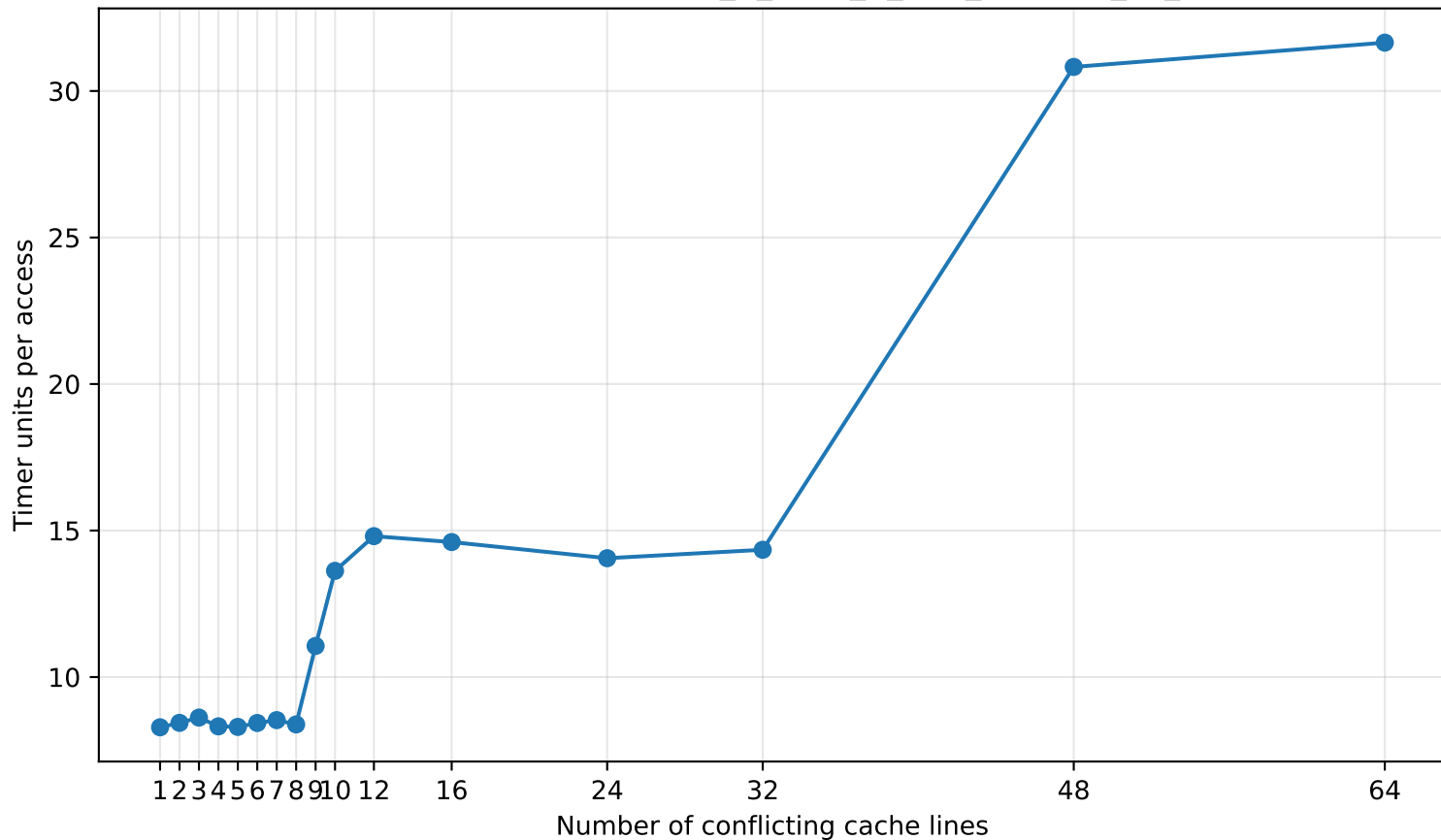
Hazel associativity sweep: Intel_R_Xeon_R_CPU_E5-2650_v4_2.20GHz
