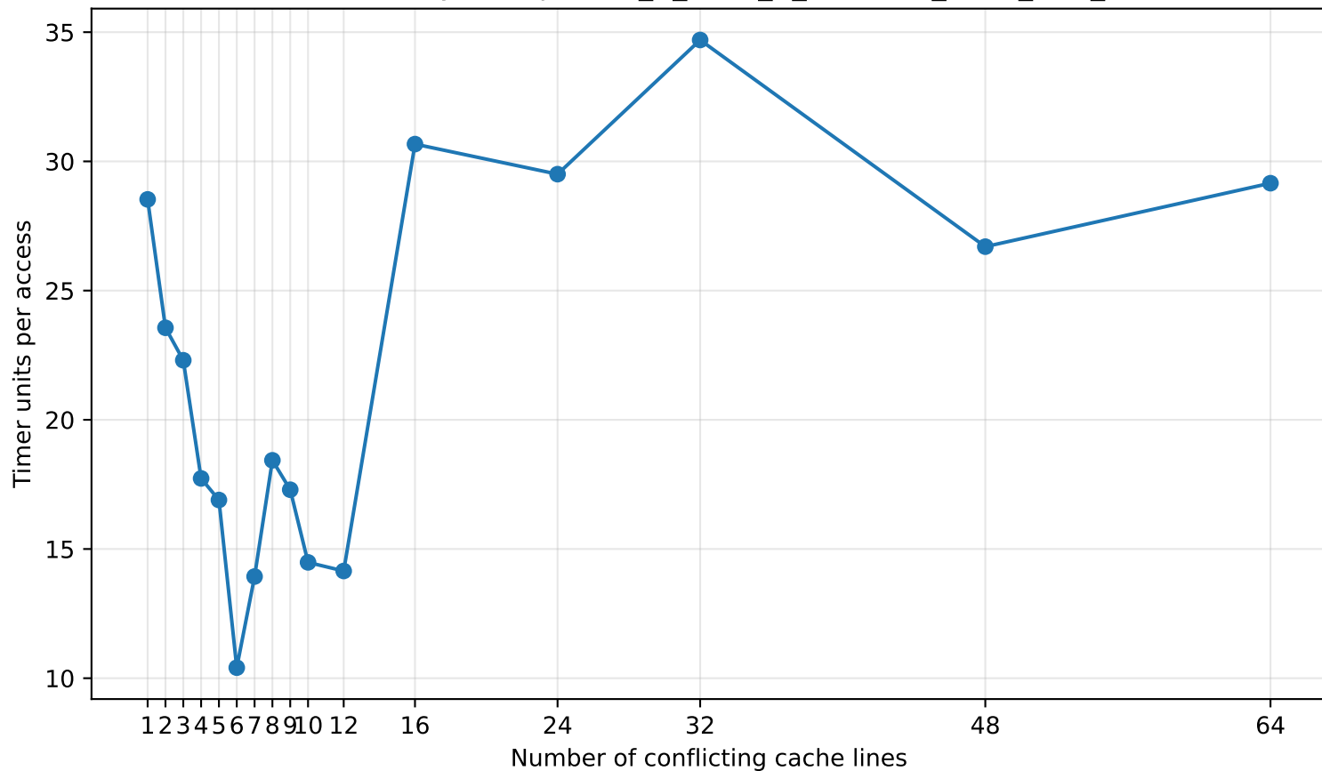
Hazel associativity sweep: Intel_R_Xeon_R_Platinum_8358_CPU_2.60GHz
