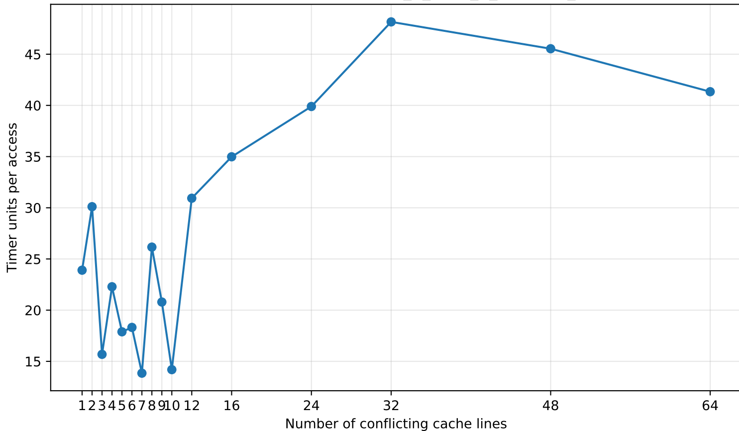
Hazel associativity sweep: Intel_R_Xeon_R_Platinum_8462Y+
