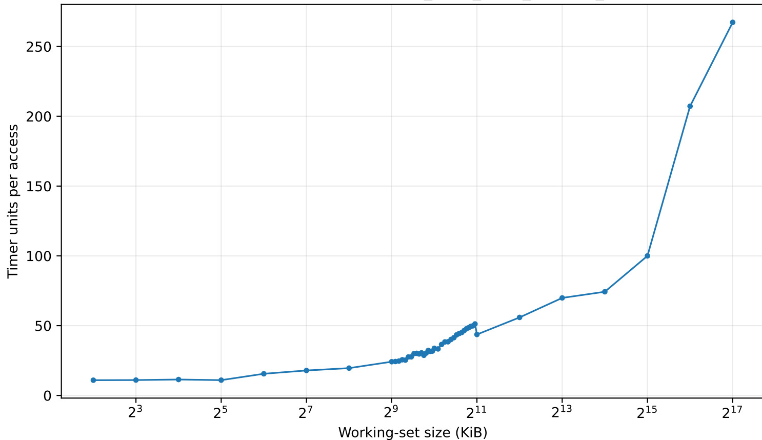
Hazel cache-capacity timing: AMD_EPYC_9654_96-Core_Processor
