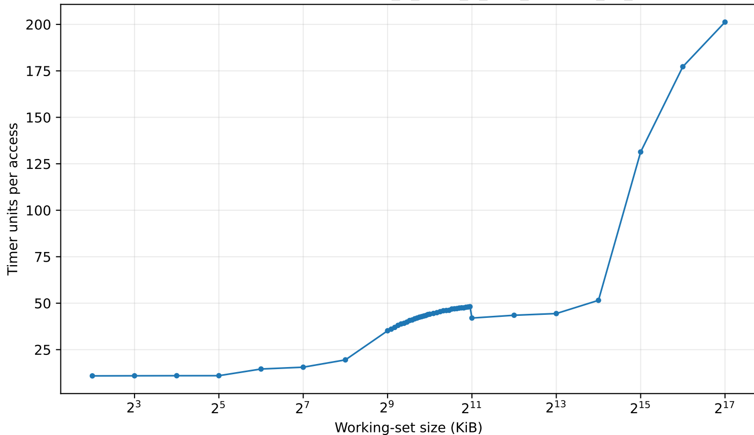
Hazel cache-capacity timing: Intel_R_Xeon_R_CPU_E5-2650_v3_2.30GHz
