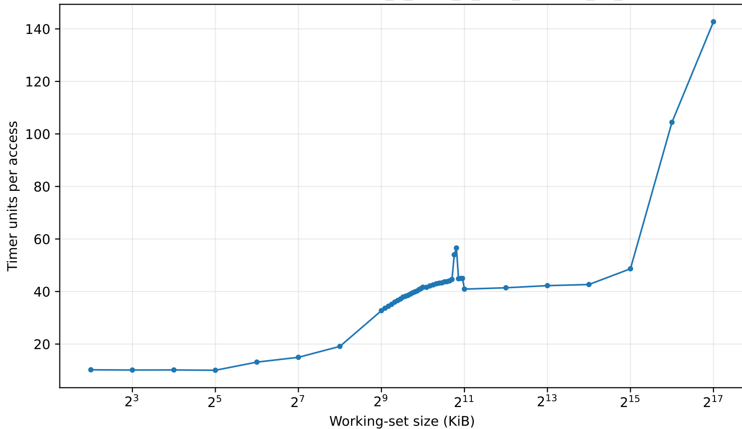
Hazel cache-capacity timing: Intel_R_Xeon_R_CPU_E5-2650_v4_2.20GHz
