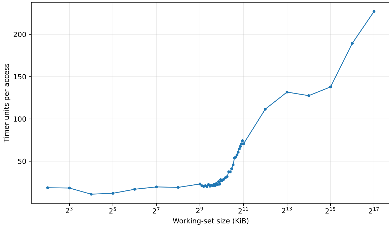
Hazel cache-capacity timing: Intel_R_Xeon_R_Gold_6326_CPU_2.90GHz
