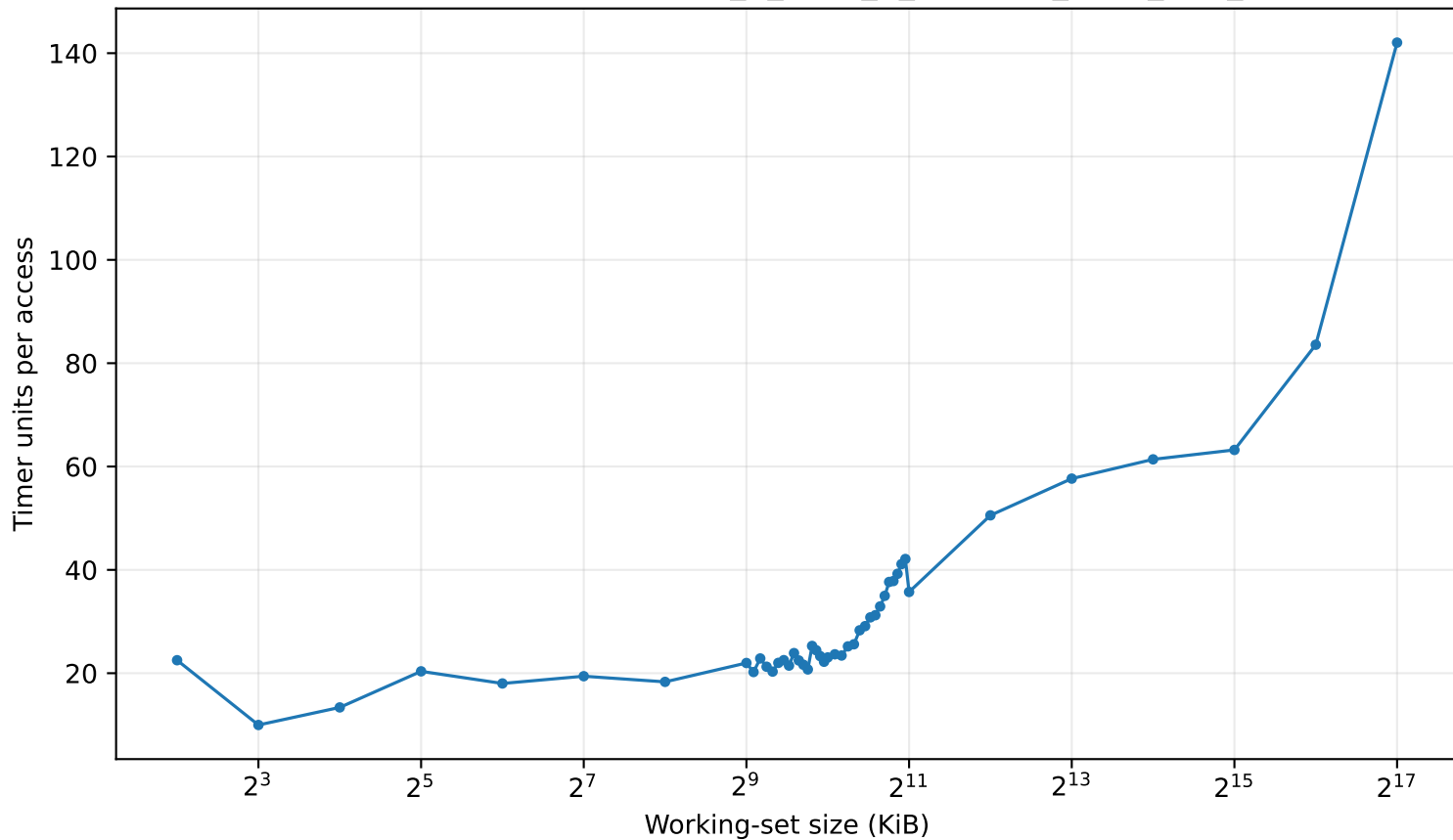
Hazel cache-capacity timing: Intel_R_Xeon_R_Platinum_8358_CPU_2.60GHz
