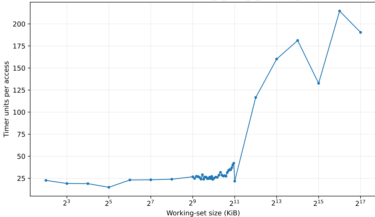
Hazel cache-capacity timing: Intel_R_Xeon_R_Platinum_8462Y+
