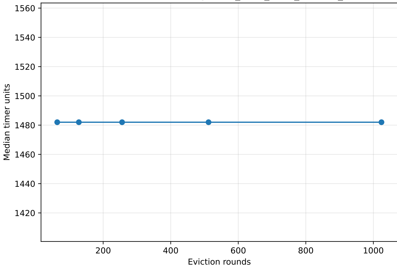
Hazel inclusion/exclusion timing: AMD_EPYC_9655_96-Core_Processor
