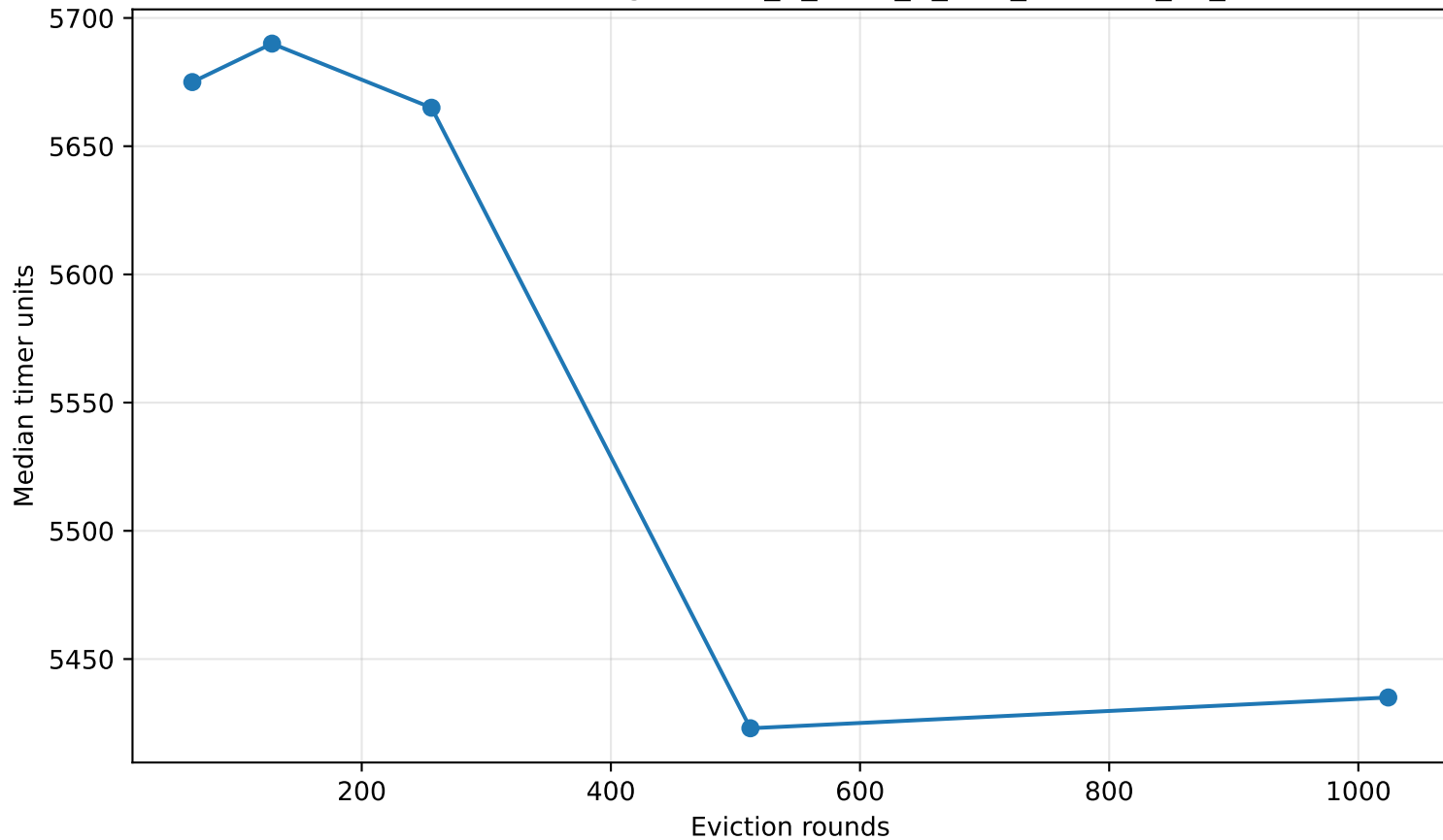
Inclusion / exclusion timing — Intel_R_Xeon_R_CPU_E5-2650_v4_2.20GHz
