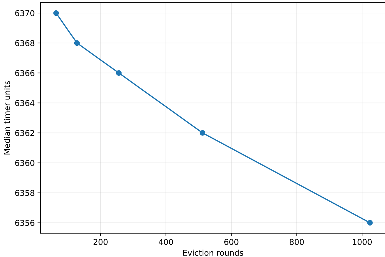
Hazel inclusion/exclusion timing: Intel_R_Xeon_R_Gold_6326_CPU_2.90GHz
