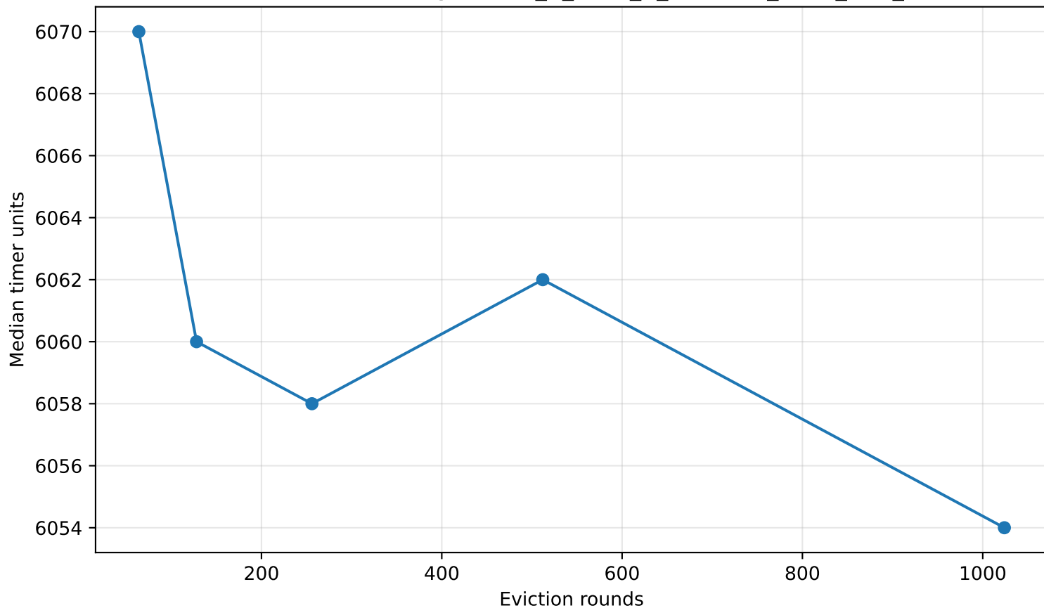
Inclusion / exclusion timing — Intel_R_Xeon_R_Platinum_8358_CPU_2.60GHz
