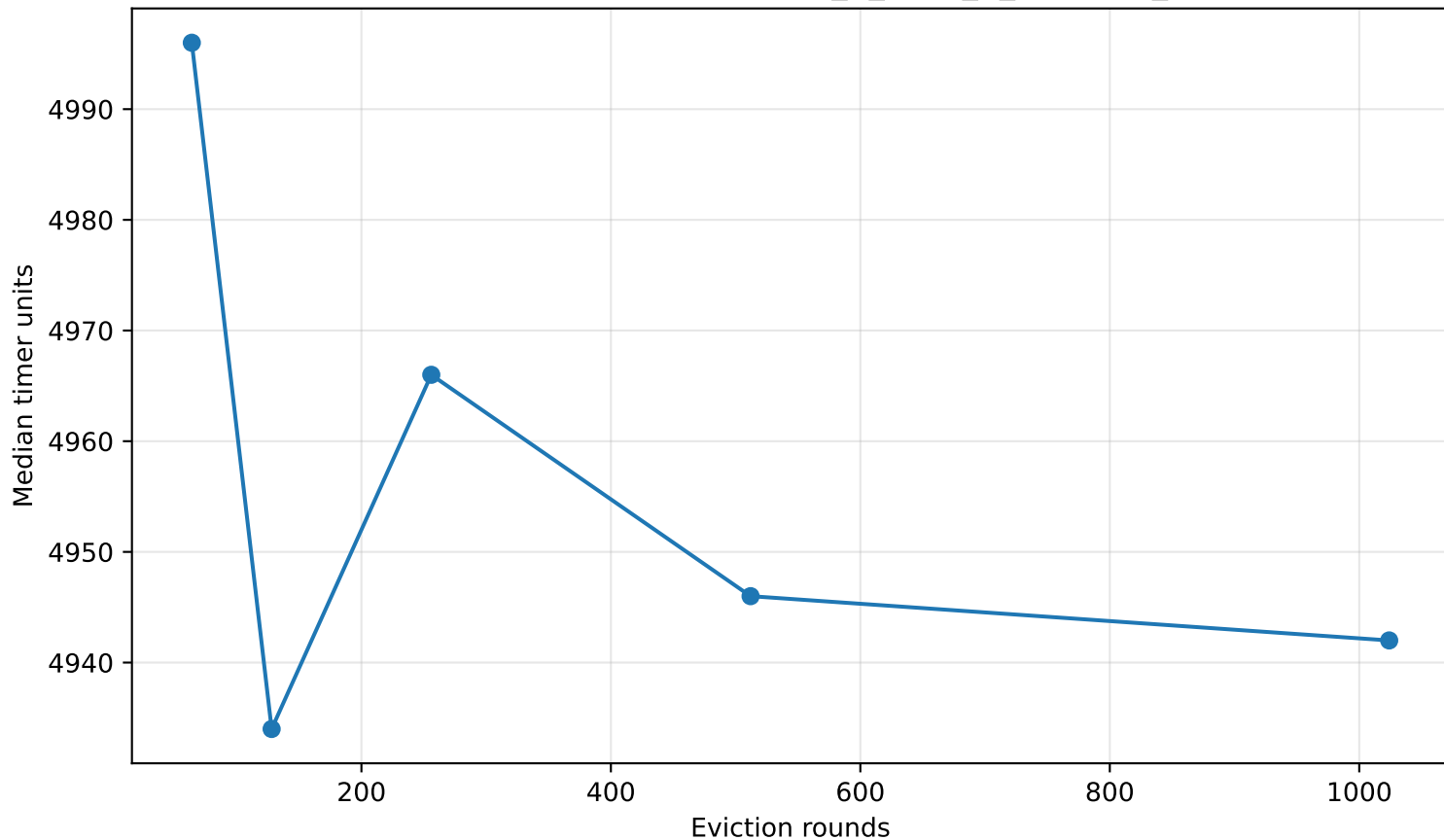
Inclusion / exclusion timing — Intel_R_Xeon_R_Platinum_8462Y+
