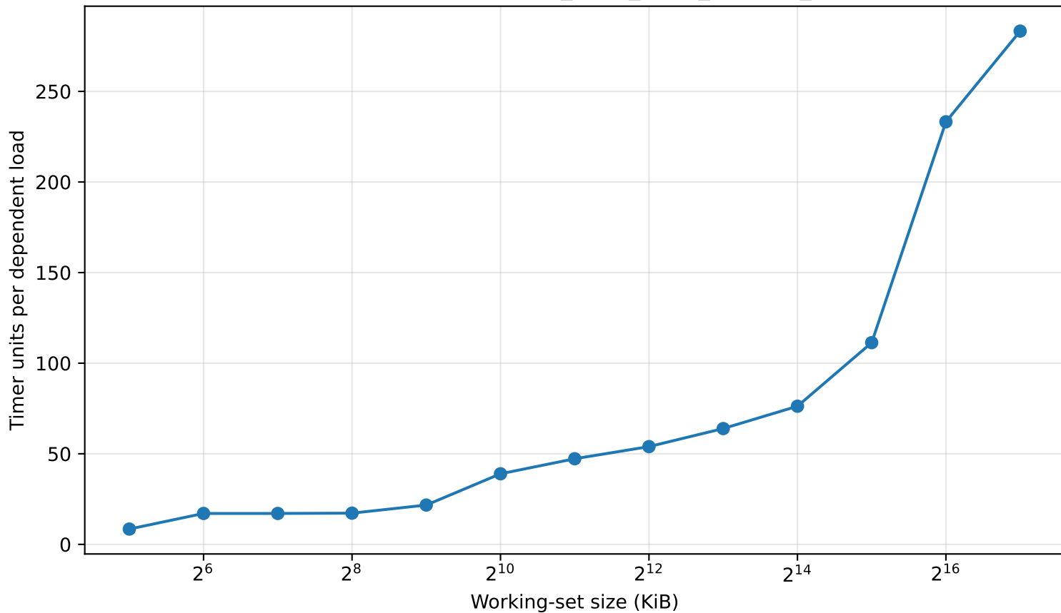
Cache latency sweep — AMD_EPYC_9654_96-Core_Processor
