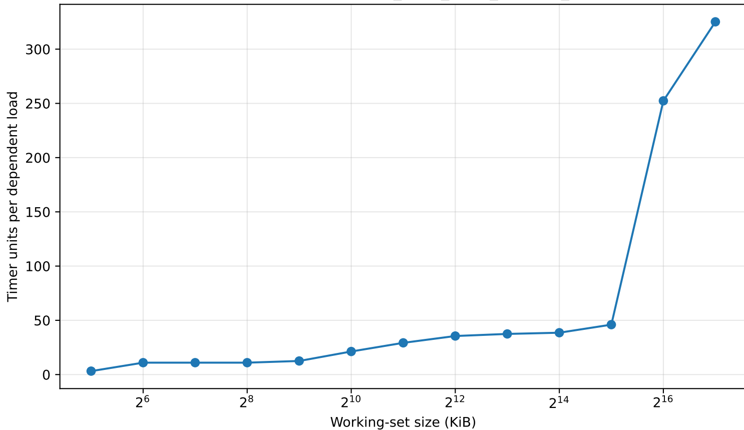
Cache latency sweep — AMD_EPYC_9655_96-Core_Processor
