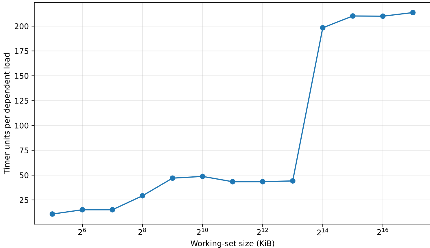
Cache latency sweep — Intel_R_Xeon_R_CPU_E5-2650_v3_2.30GHz
