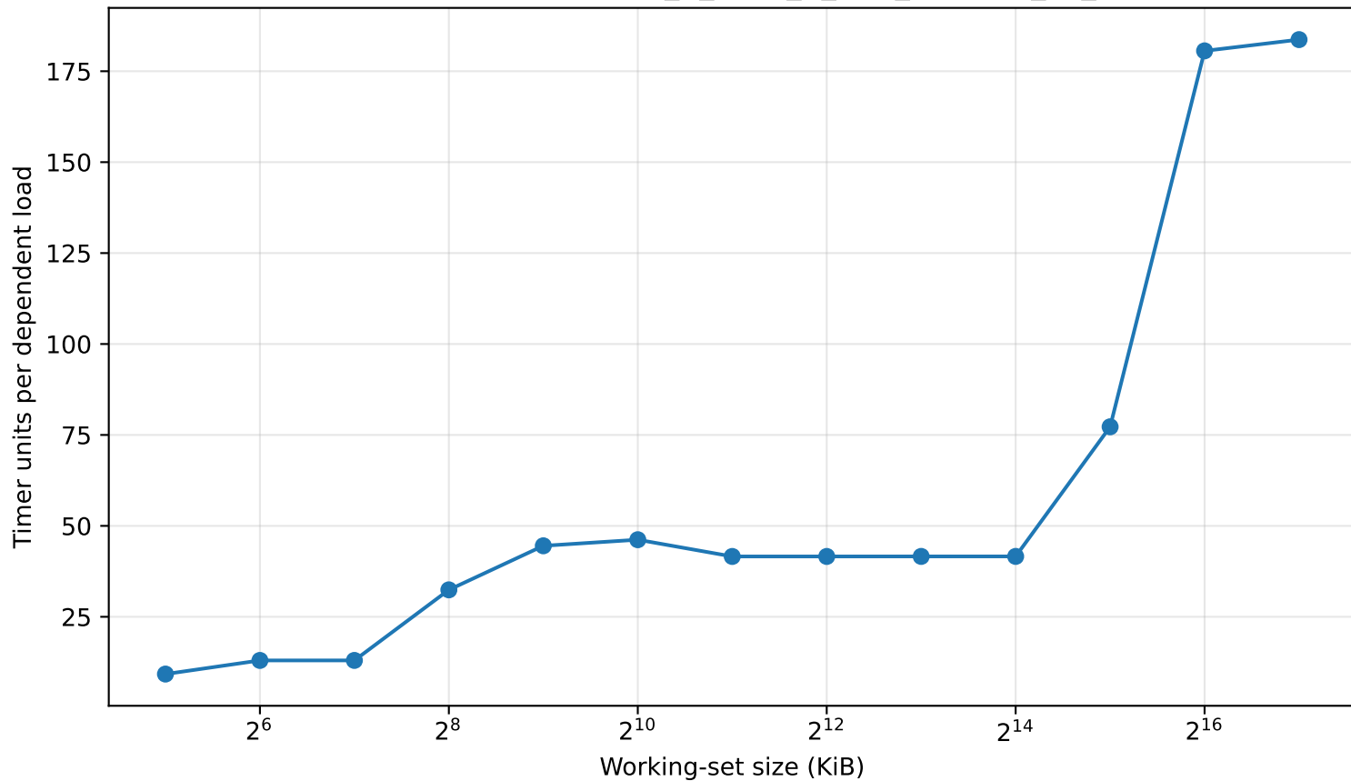
Cache latency sweep — Intel_R_Xeon_R_CPU_E5-2650_v4_2.20GHz
