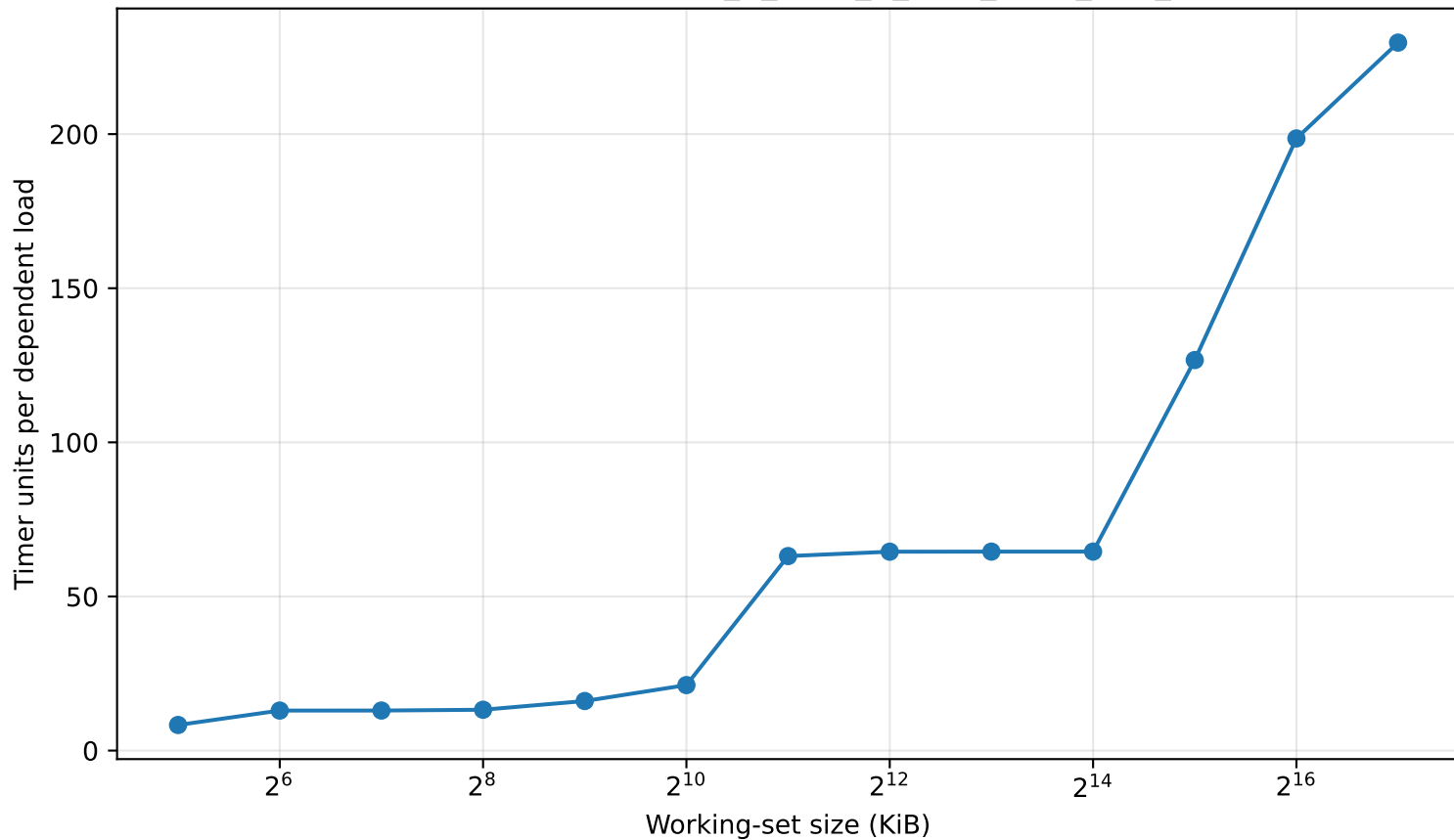
Cache latency sweep — Intel_R_Xeon_R_Gold_6326_CPU_2.90GHz
