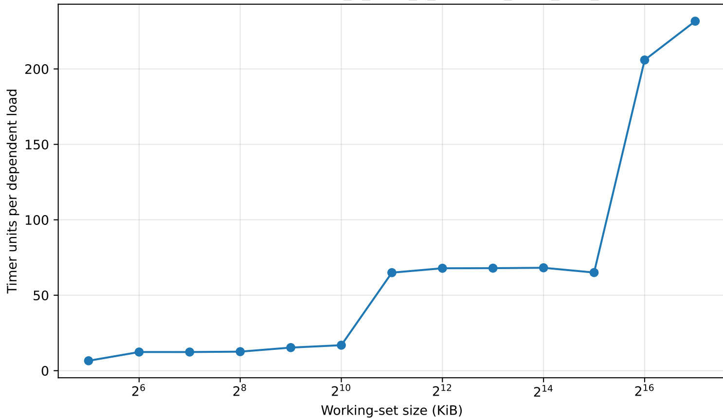
Cache latency sweep — Intel_R_Xeon_R_Platinum_8358_CPU_2.60GHz
