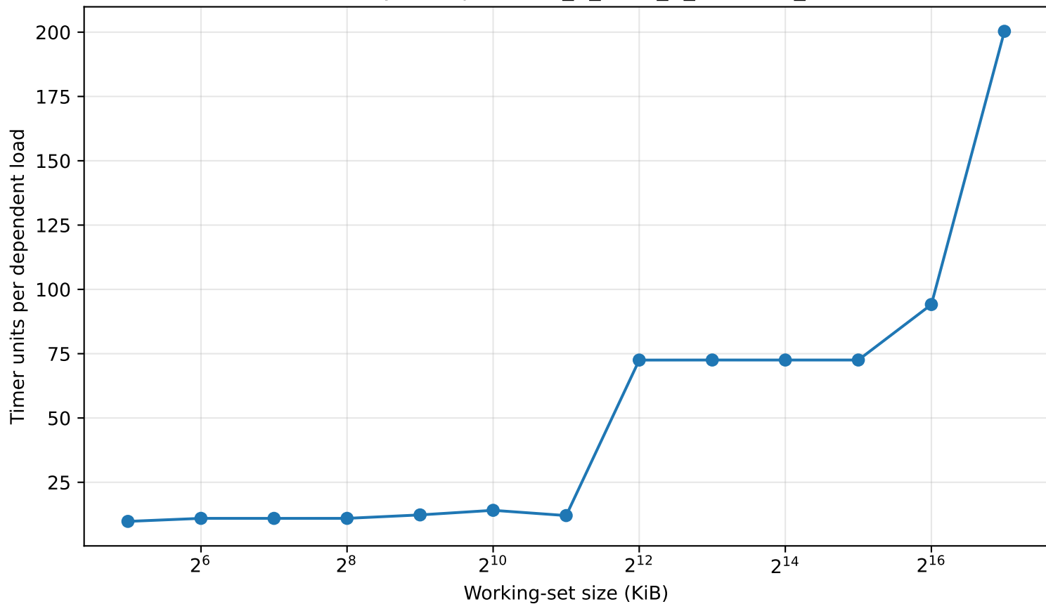
Cache latency sweep — Intel_R_Xeon_R_Platinum_8462Y+
