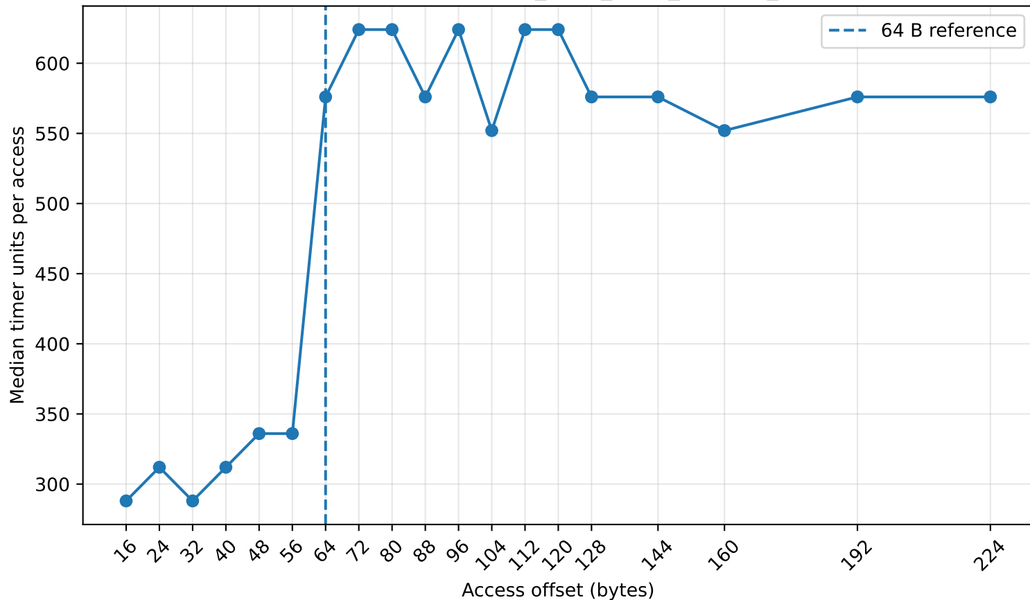
Hazel line-size sweep: AMD_EPYC_9654_96-Core_Processor
