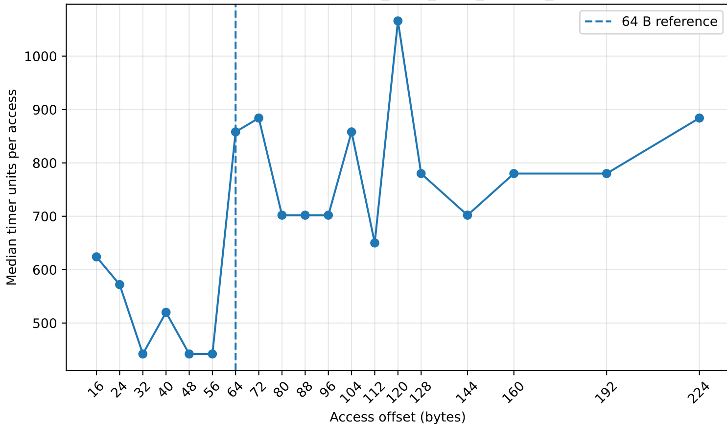
Hazel line-size sweep: AMD_EPYC_9655_96-Core_Processor
